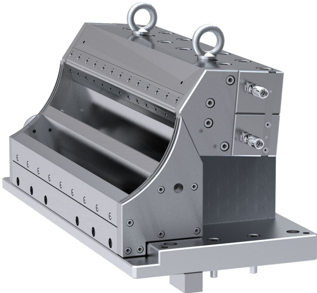
Single Layer Slot Bead Die with Vacuum Box
